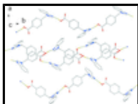
Fig. 2. The packing diagram of the title compound. Hydrogen bonds are shown as dashed lines.
